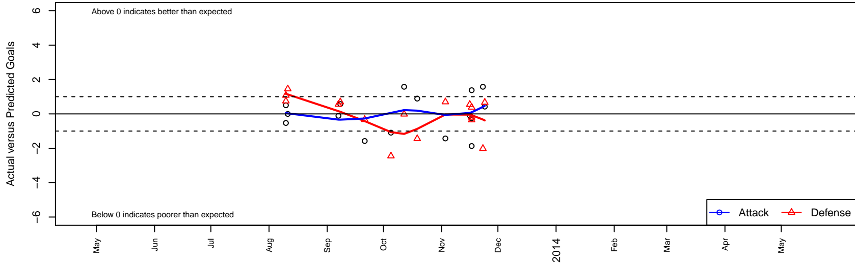
Barcelona Bay Area Fusion G99 Dots are actual minus expected GF (blue circles) and GA (red triangles). Blue line is smoothed change in attack strength. Red is smoothed change in defense strength.
